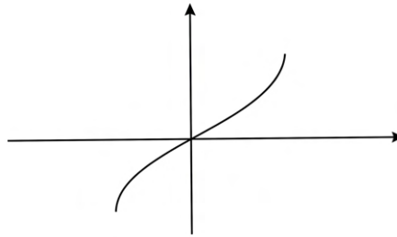
Unstable Vacuum
