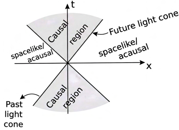
Figure: Light Cone
