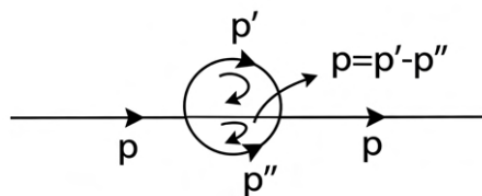
2-loop indendepnt momenta
