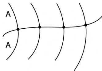
fiber bundles
